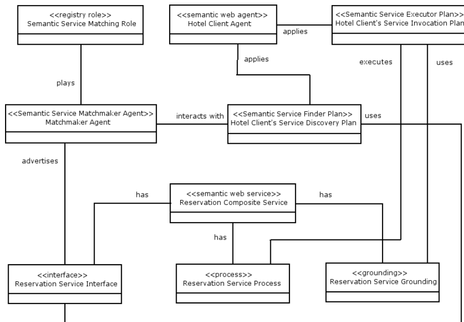
Figure 7: An instance model for the agent – service interaction within a MAS working in Tourism domain
