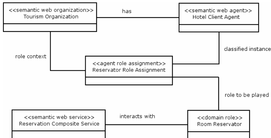
Figure 5: A Semantic Role Assignment for a MAS working in Tourism domain.
