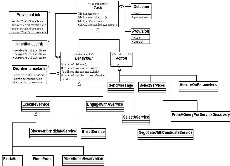
Figure 9: An instance plan model in SEAGENT for the agent – service interaction within a MAS working in Tourism domain
