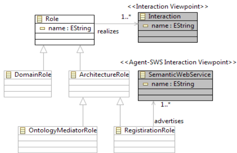
Figure 4: Role viewpoint.
