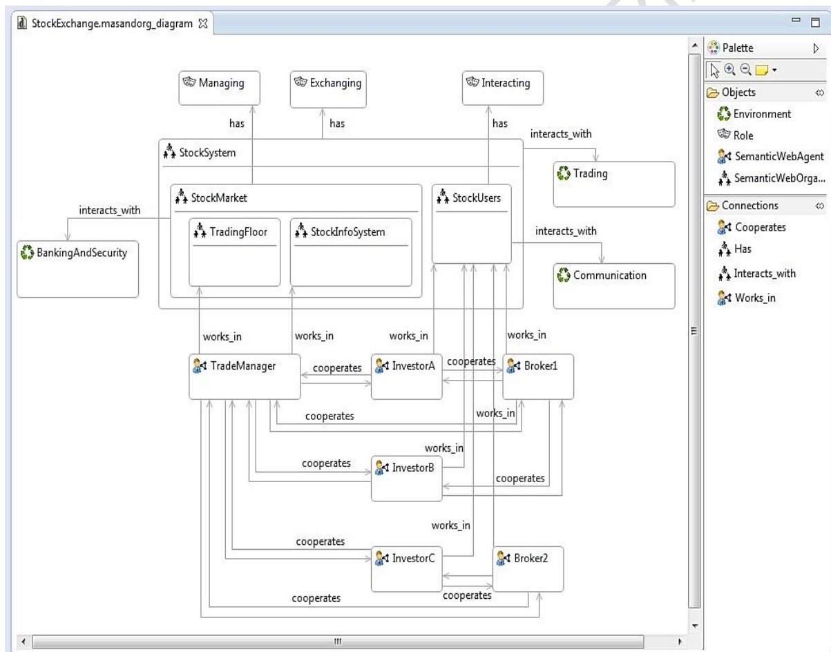
Figure 12: Graphical modeling for the MAS viewpoint of the Stock Exchange system in the SEA_ML graphical syntax tool
