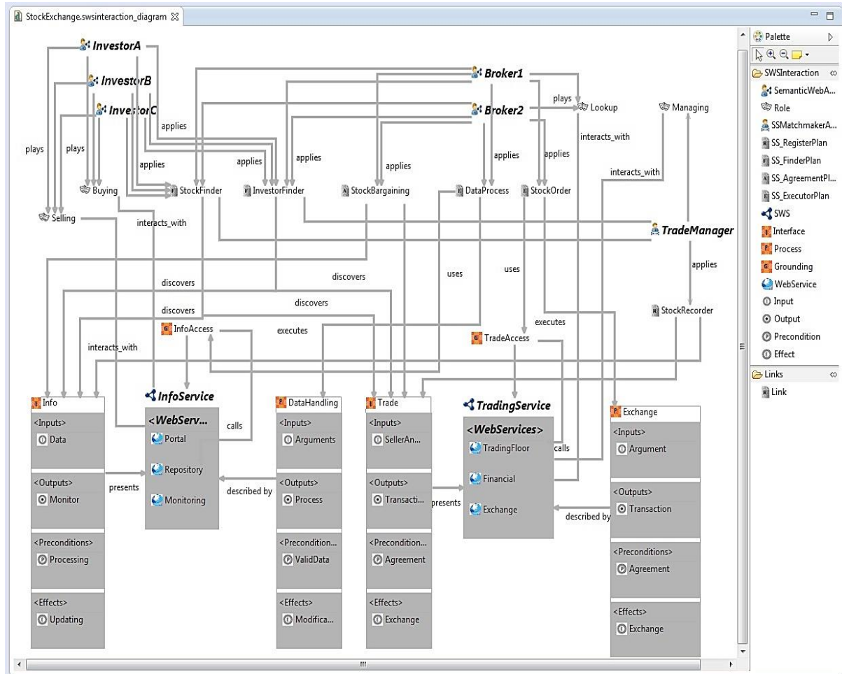
Figure 14: Graphical modeling for the agent-SWS Interaction viewpoint of a multi-agent stock exchange system in the graphical syntax tool of SEA_ML
