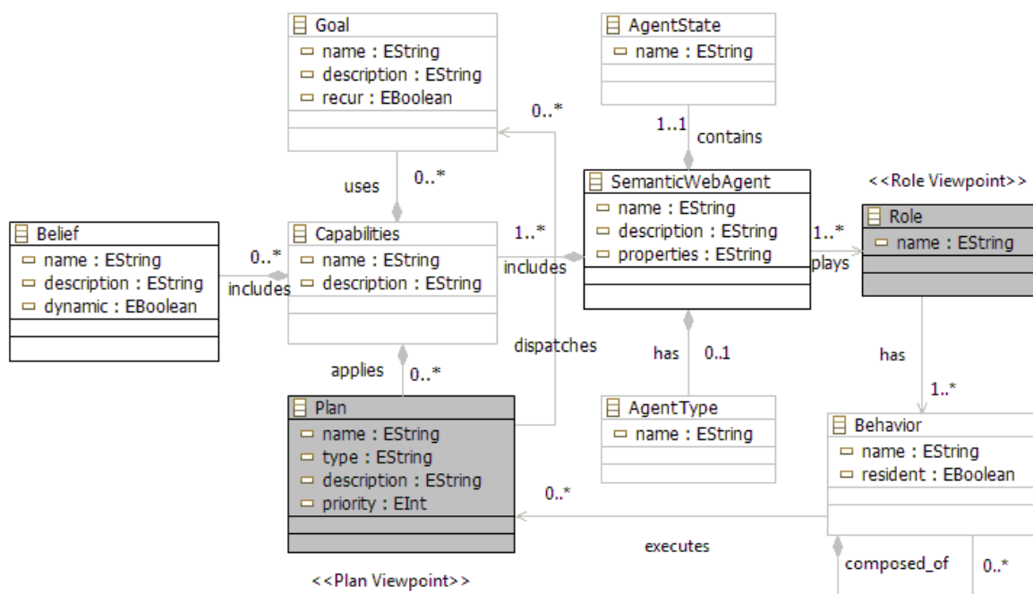
Figure 2: Agent Internal viewpoint.
