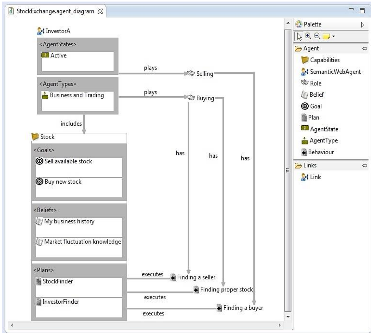
Figure 13: Graphical modeling for the agent internal viewpoint of a multi-agent stock exchange system in the graphical syntax tool of SEA_ML
