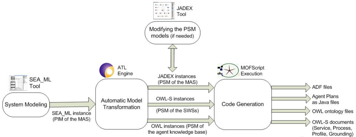
Figure 10: SEA_ML-based MAS development methodology
