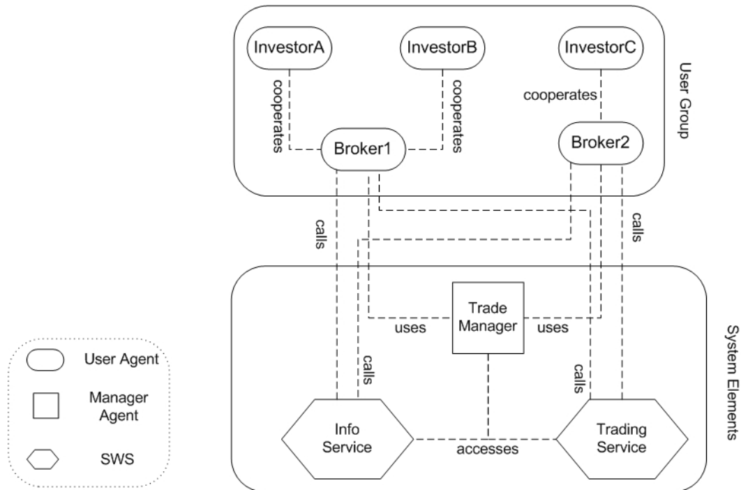
Figure 11: Architecture of the Stock Exchange case study
