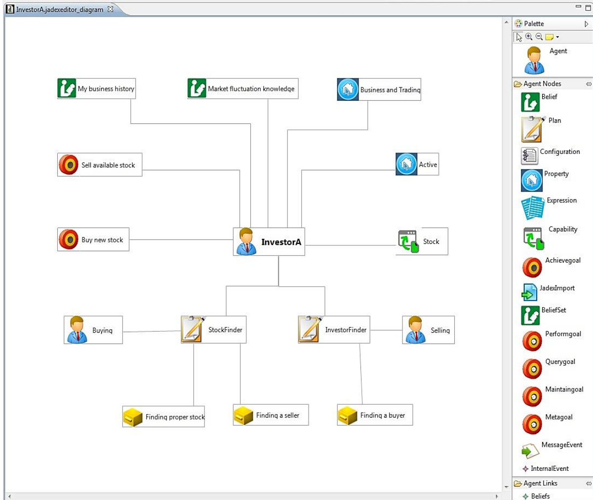
Figure 15: Partial graphical model of the transformed agent internal viewpoint inside the platform-specific modeling tool (Kardas et al., 2009b) for JADEX agents
