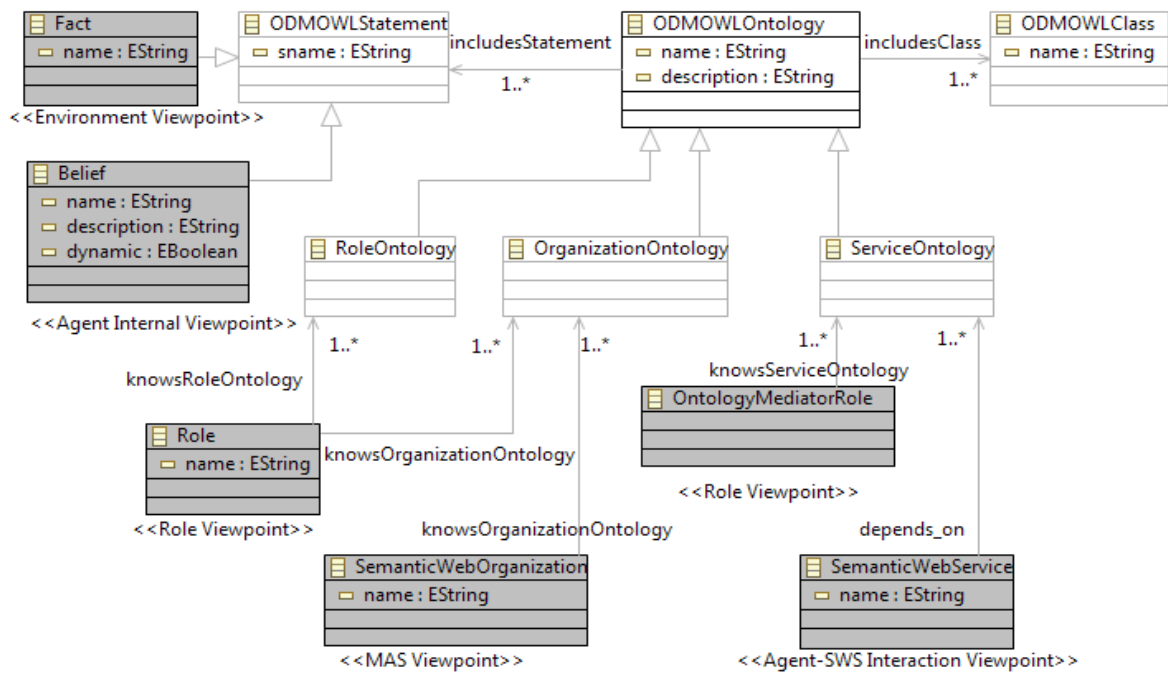
Figure 8: Ontology viewpoint.
