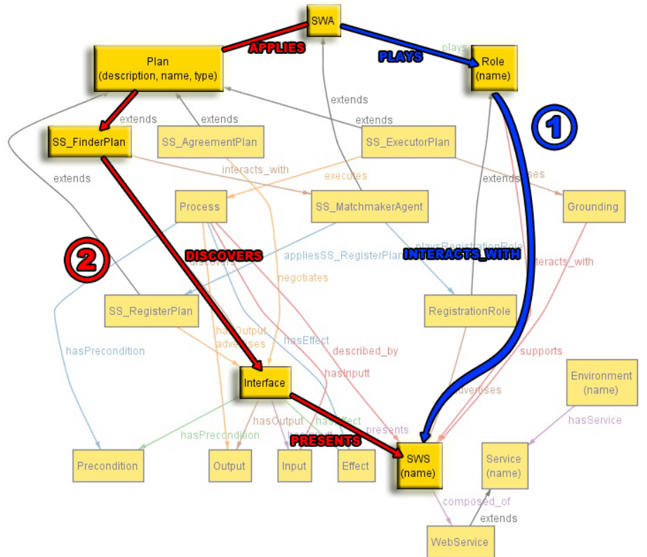
Figure 28: Agent-SWS Interaction Paths
