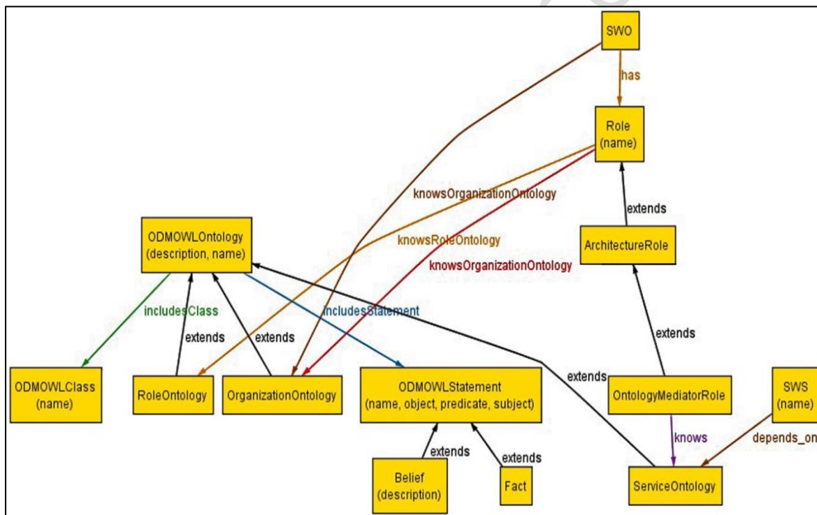
Figure 22: SEA_ML's Ontology viewpoint
