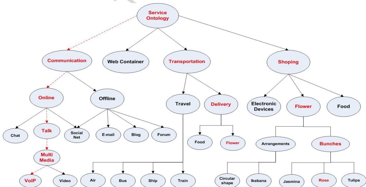
Figure 6: An example of the Service Ontology used in the expert finder system.
