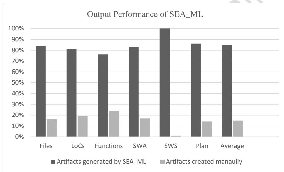
Diagram 1. Output performance of SEA_ML
