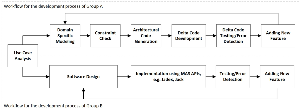
Figure 4. The workflow representing steps of the development for Group A and Group B
