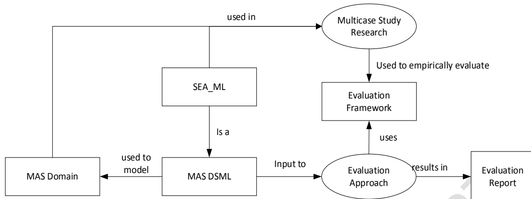
Figure 2. Conceptual model of the DSML evaluation approach representing the context of the framework
