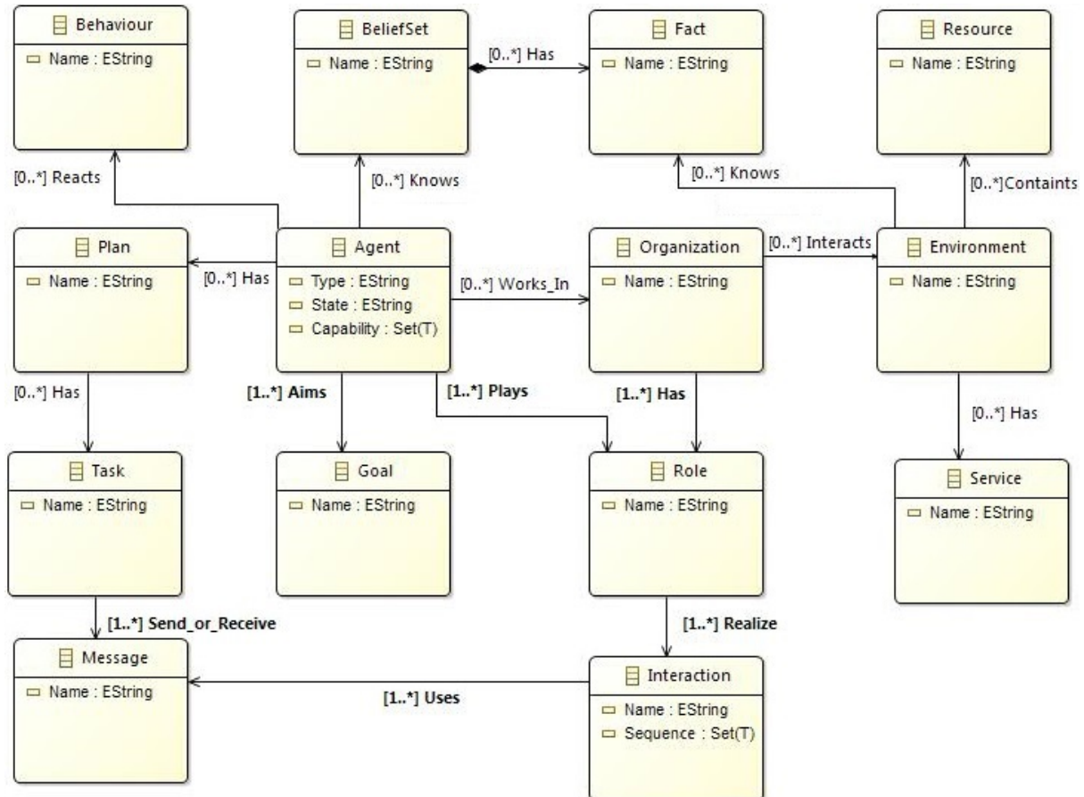
Figure 1. General metamodel (abstract syntax) representing MAS DSMLs
