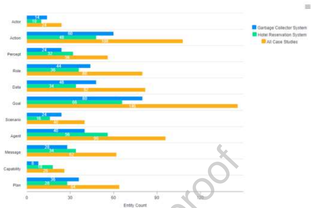
Figure 4.8: The usage frequencies of PDT language elements during multi-case studies
